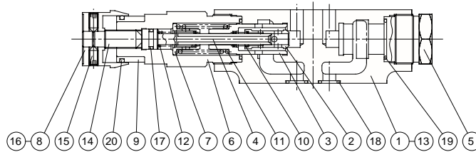
Seal Part List (Kit Model Number BFCS-01CF*)
